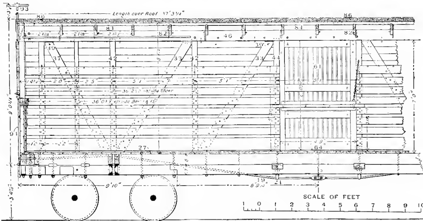
Fig. 371. Part Longitudinal Section.
